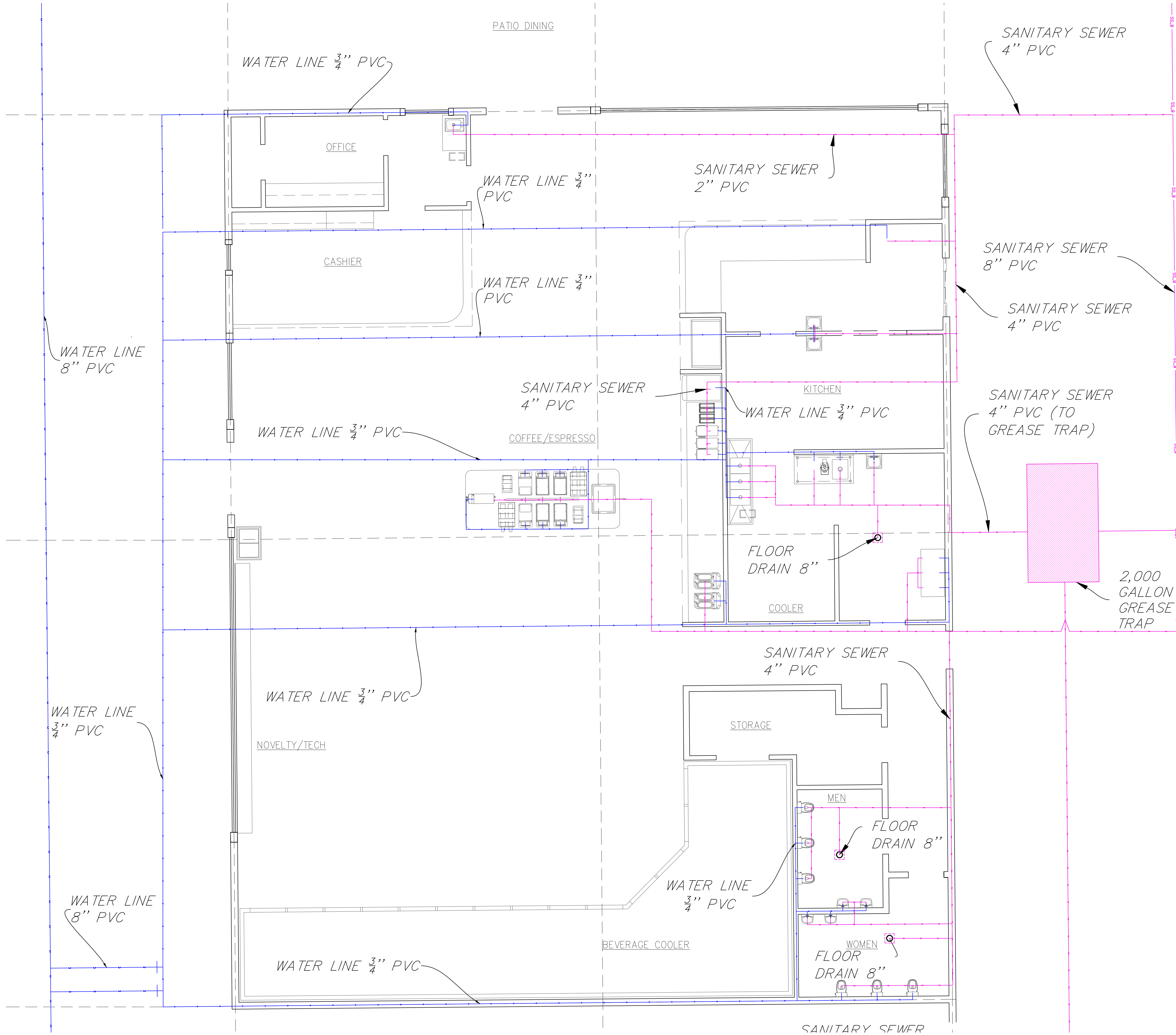
1 PLUMBING PLAN CONVENIENCE STORE P1.02 SCALE: 1/4" = 1'
